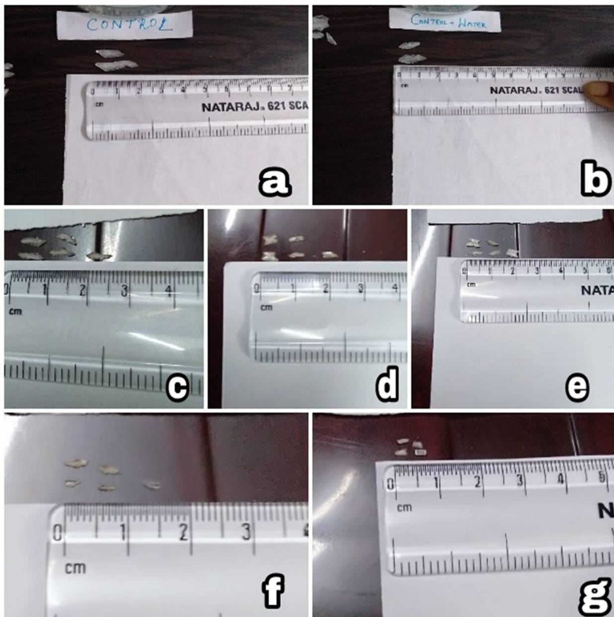
Fig. 3: The measurement of struvite obtained from Alpinia calcarata stem in the gel method (a) without any additive (b) with the distilled water (c) with the 0.15% of methanol extract (d) with the 0.25% of methanol extract (e) with the 0.50% of methanol extract (f) with the 0.75% of methanol (g) with the 1.00% of methanol extract.
