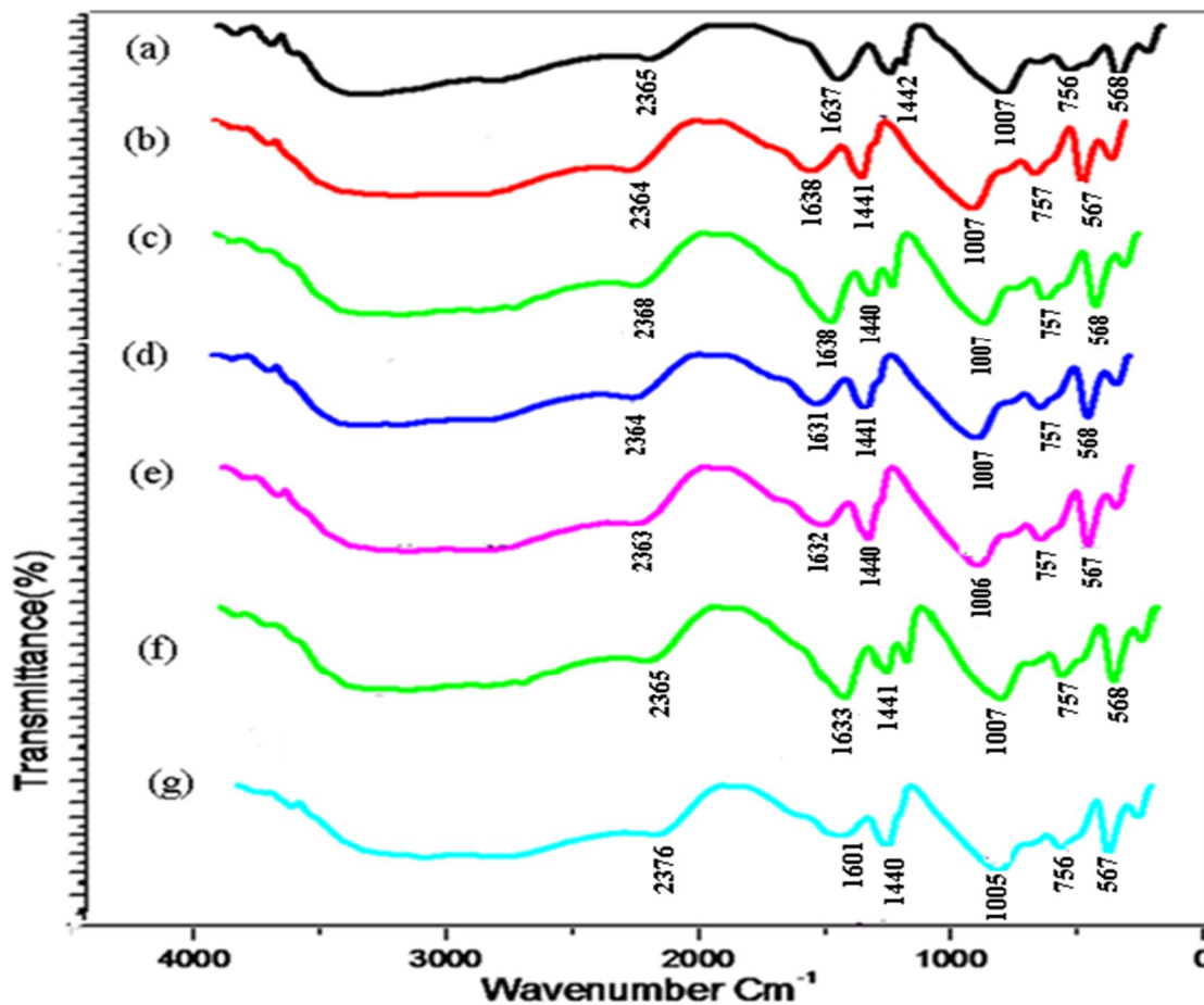
Fig. 4: The FTIR spectra of struvite obtained from Alpinia calcarata stem in the gel method (a) without any additive (b) with the distilled water (c) with the 0.15% of methanol extract (d) with the 0.25% of methanol extract (e) with the 0.50% of methanol extract (f) with the 0.75% of methanol extract (g) with the 1.00% of methanol extract.
