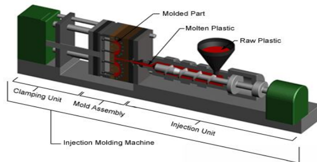
Fig 1. Injection Molding Machine
