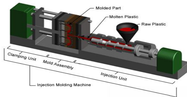
Fig 1. Injection Molding Machine
