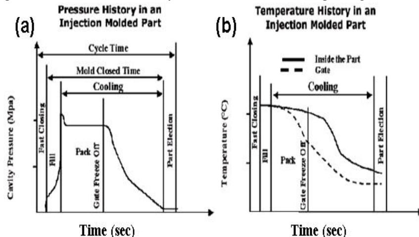
Fig. 2. Pressure And Temperature Cycle of Injection Molding
