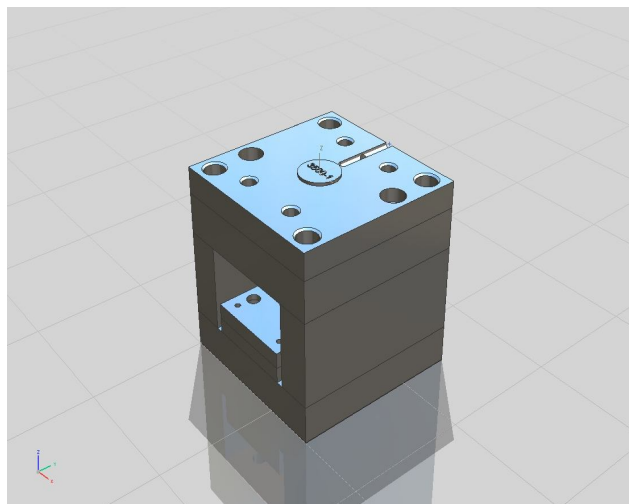
Fig.4. Optimized Mold Structure
