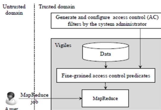
Figure 13: Vigiles access control mechanism.
