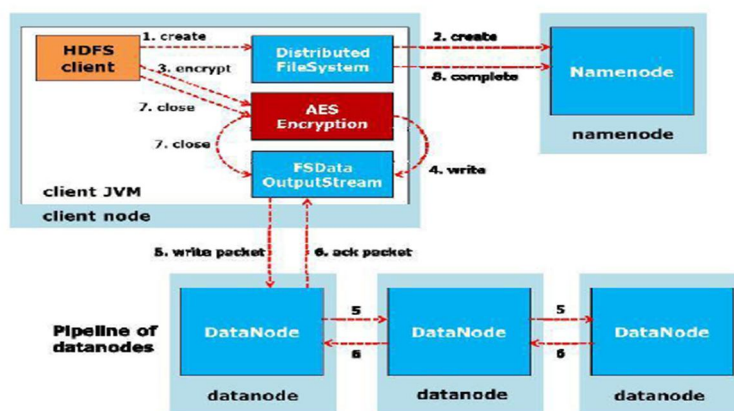
Figure 11: Encryption Process
