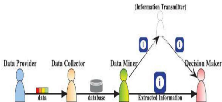
Figure 15: Application Scenario.
