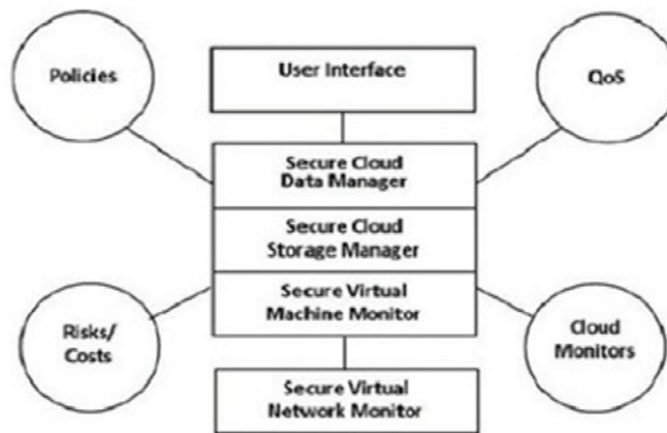
Figure 10: Layered Framework for Assuring Cloud
