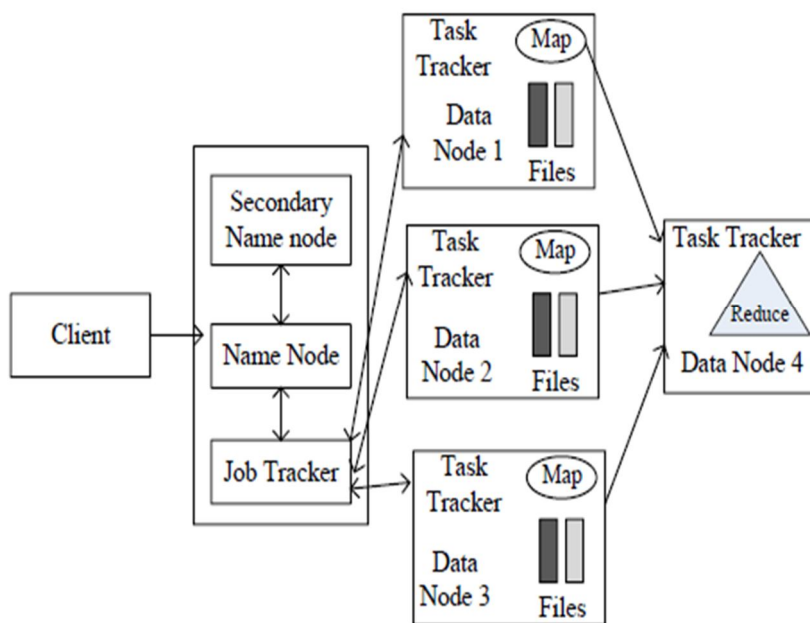
Figure 7: Hadoop based on MapReduce paradigm
