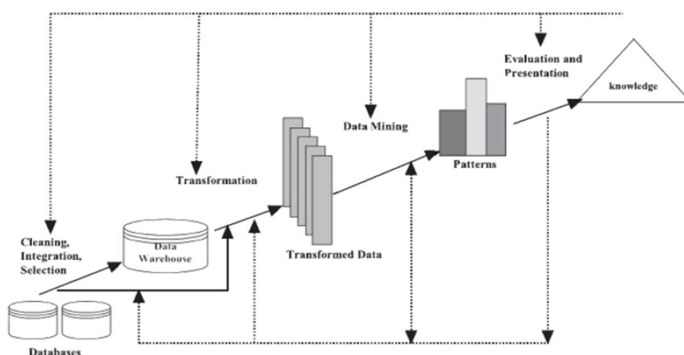
Figure 4: Knowledge-Discovery Process
