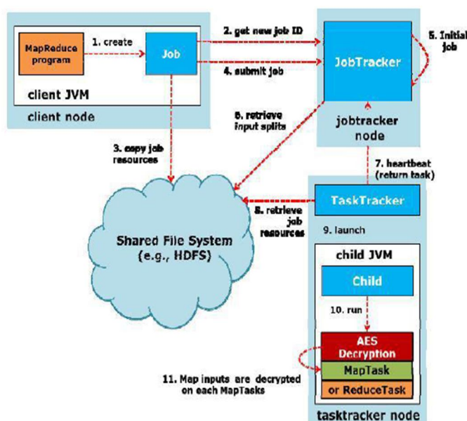
Figure 12: Decryption Process
