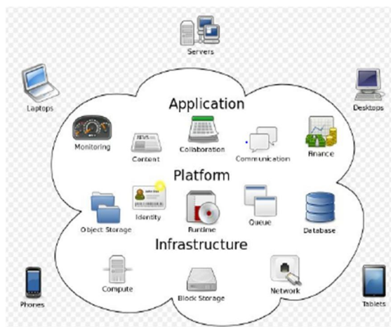
Figure 3: Cloud Computing
