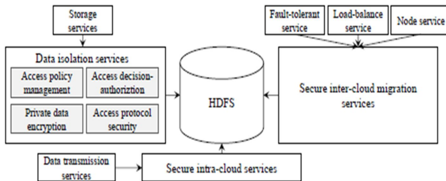
Figure 14: SAPSC architecture for data security.
