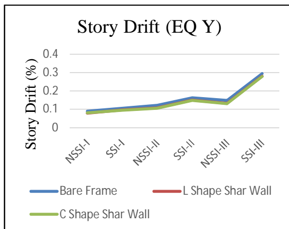
Figure 6.4: Comparison of Story Drift in EQ – X & EQ - Y for Model 1, 2 & 3
