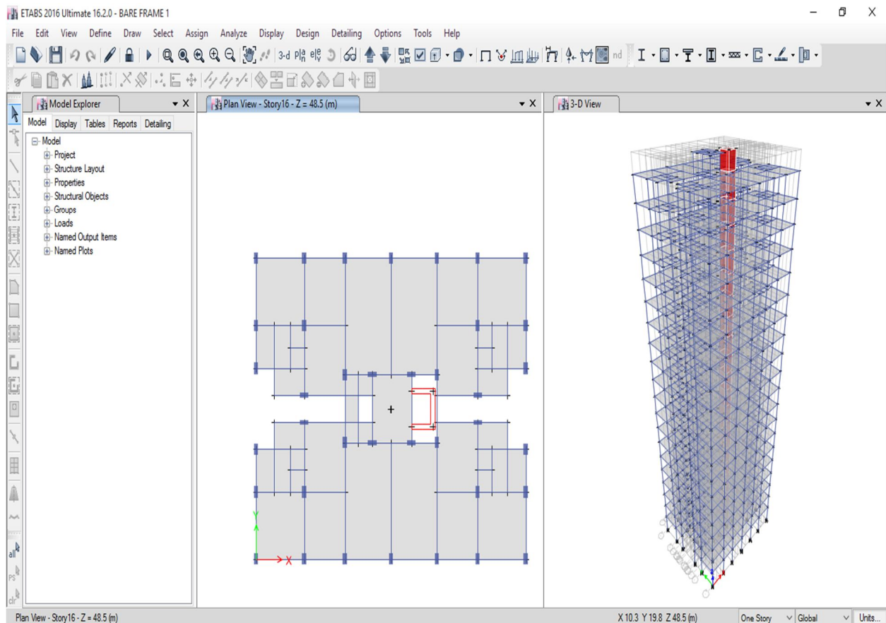
Figure 5.1: RCC Bare Frame Structure (Model 1)
