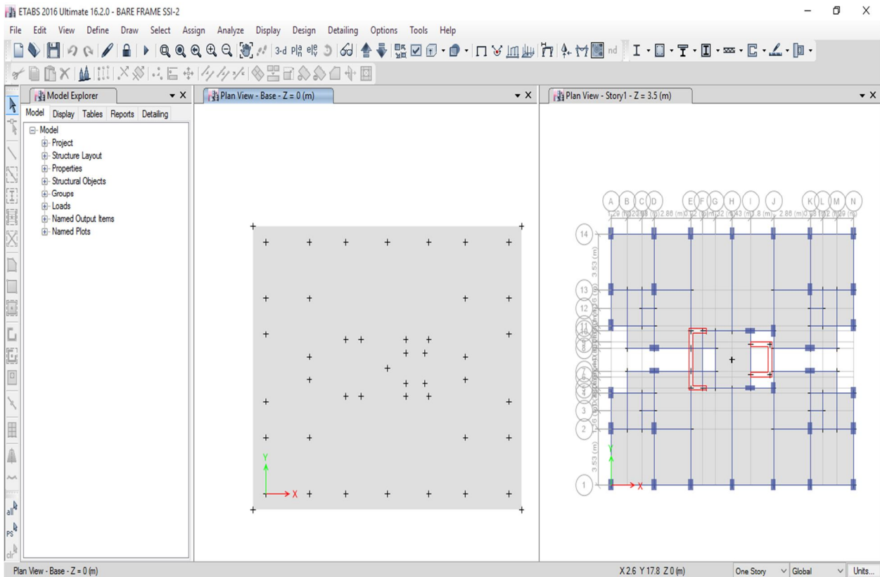
Figure 5.3: RCC Bare Frame Structure C shape shear wall at core (Model 3)
