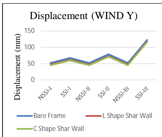
Figure 6.3: Comparison of Roof Displacement in Wind – X & Wind - Y for Model 1, 2 & 3
