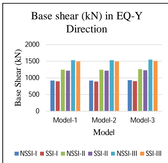
Figure 6.2: Comparison of Base Shear in EQ – X & EQ - Y Direction for Model 1, 2 & 3
