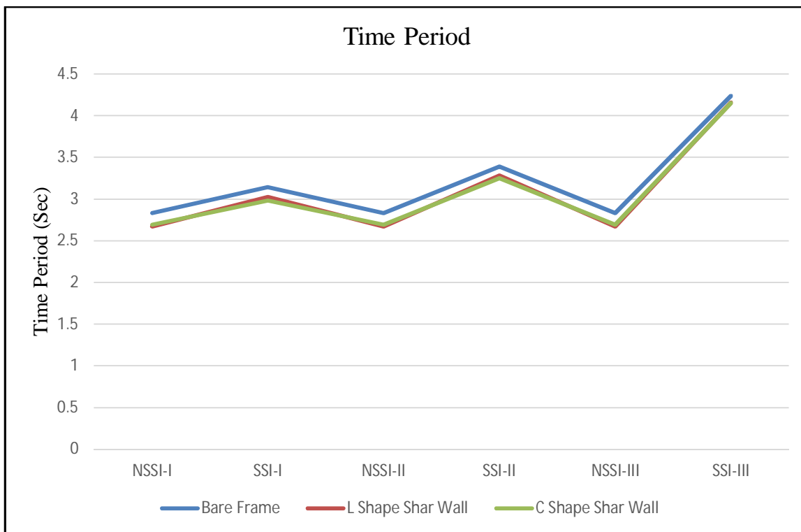
Figure 6.1: Comparison of Time Period for Model 1, 2 & 3
