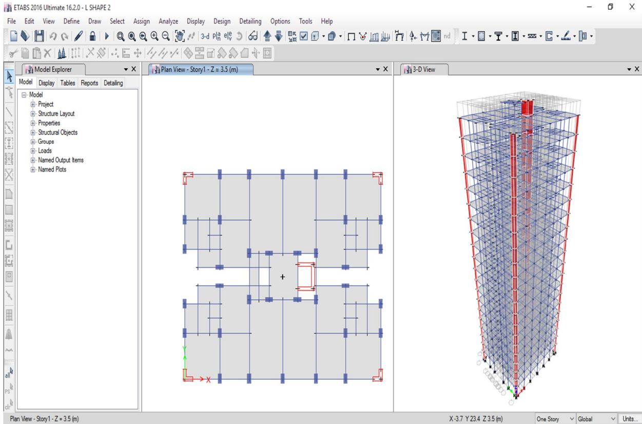
Figure 5.2: RCC Bare Frame Structure with L shape shear wall at periphery (Model 2)
