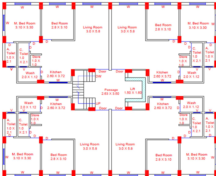
Figure 4.1: Geometry of Building Plan
