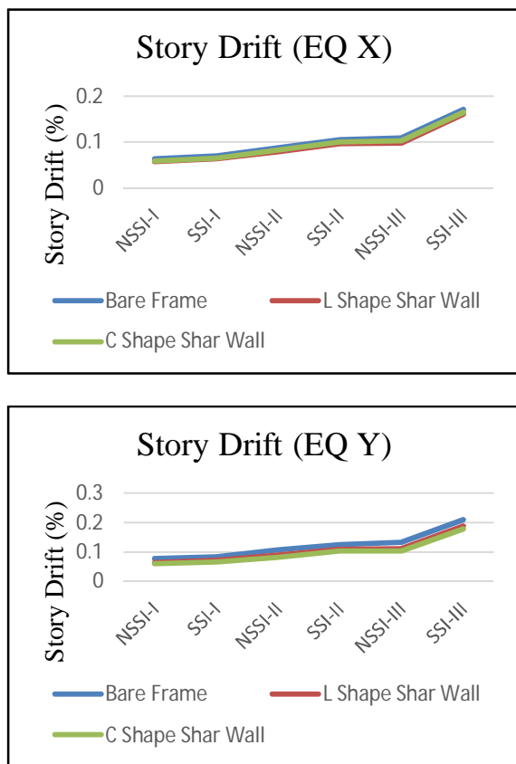
Figure 6.5: Comparison of Story Drift in EQ – X & EQ – Y for Model 1, 2 & 3
