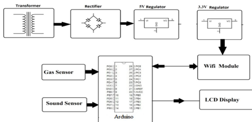
Fig. 2: Block Diagram
