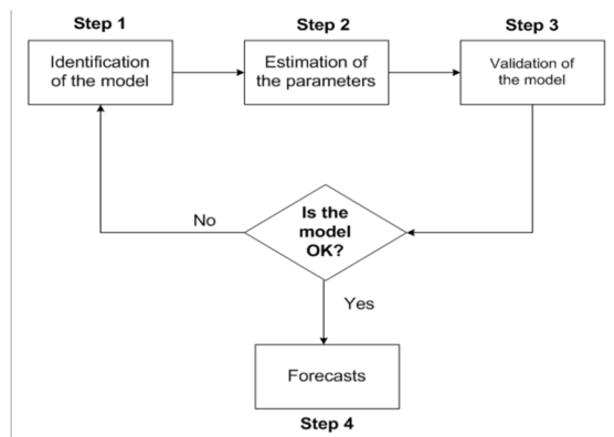
Fig: 1 Outline of Box-Jenkins Methodology.
