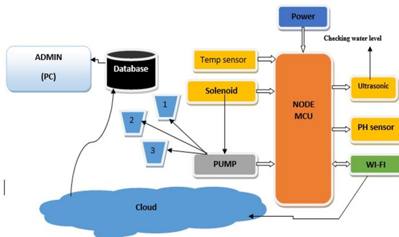
Block Diagram:
