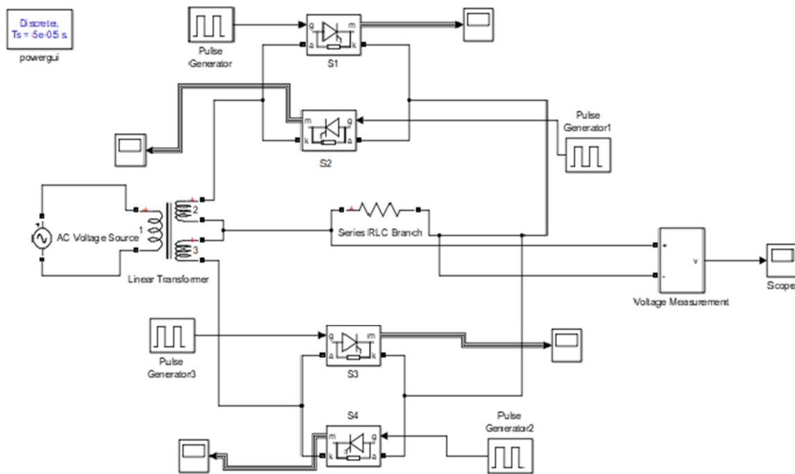
Fig 1: Simulation Circuit For CYCLO-Converter With R Load
