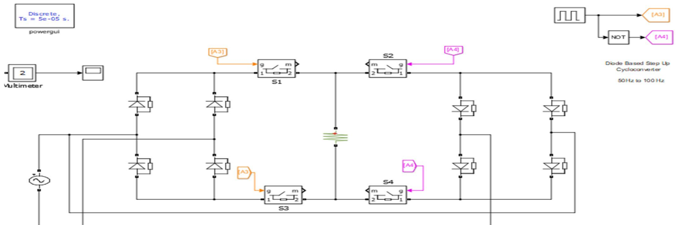
Fig 5: Simulation Circuit Of Step Up Cyclo-Converter With RL Load
