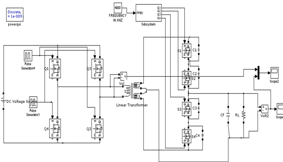
Fig 2: Simulation Circuit For Frequency Control Cyclo-Converter For 10khz
