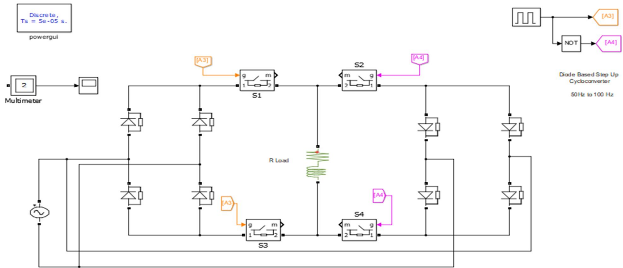
Fig 4: Simulation Circuit Of Step Up Cyclo-Converter With R Load
