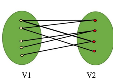
Fig 4. Bipartite graph
