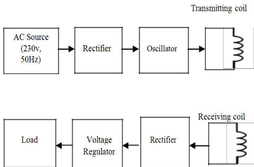
Fig. 1 Basic block diagram of a wireless power transfer
