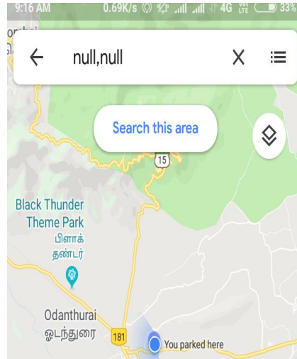
Fig 4: Mapping page
