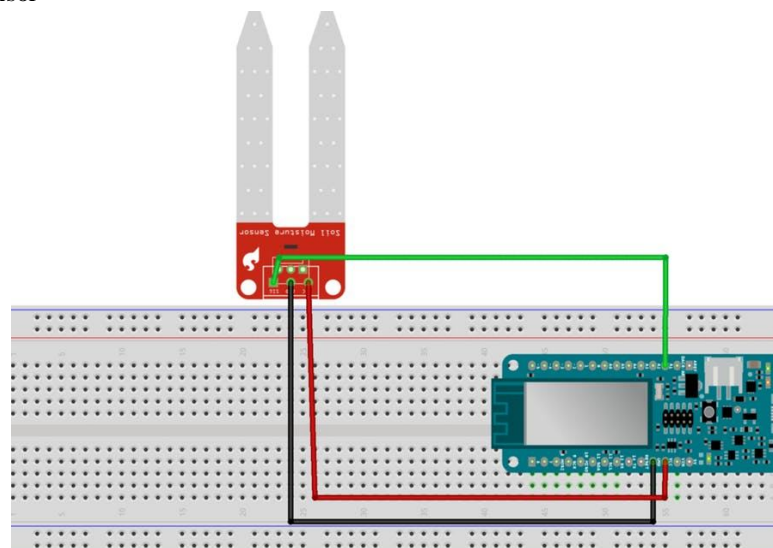
Fig.4 Soil Moisture Sensor
