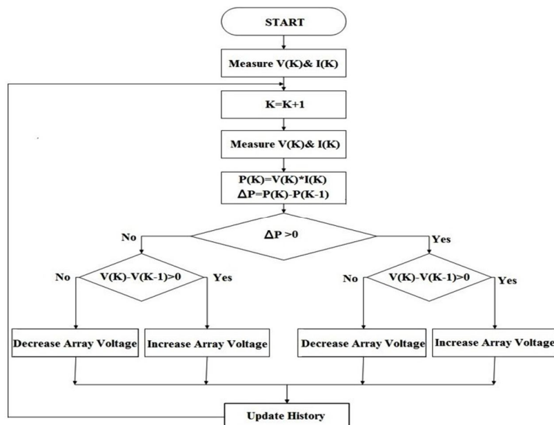
Fig. Flowchart of P&O algorithm
