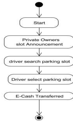
Fig. 2 Activity Diagram
