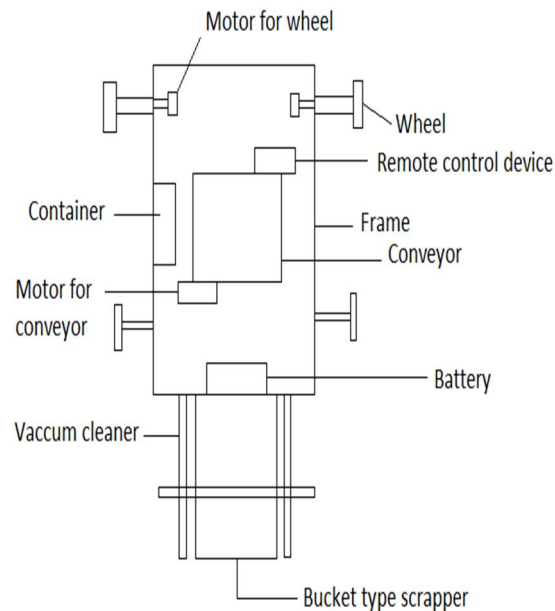
Design of scrap collecting vehicle
