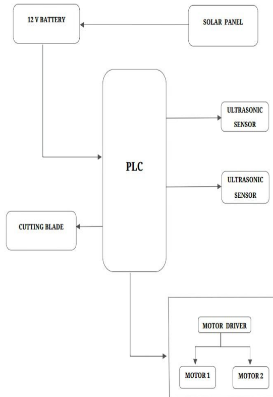
Figure 1:- Block Diagram
