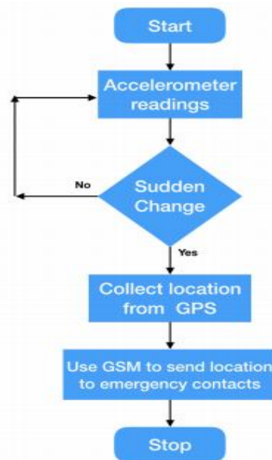
Figure 4: Flow Chart for accident detection
