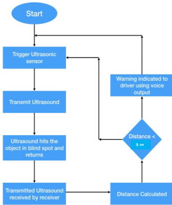
Figure 3: Flow Chart for vehicle detection
