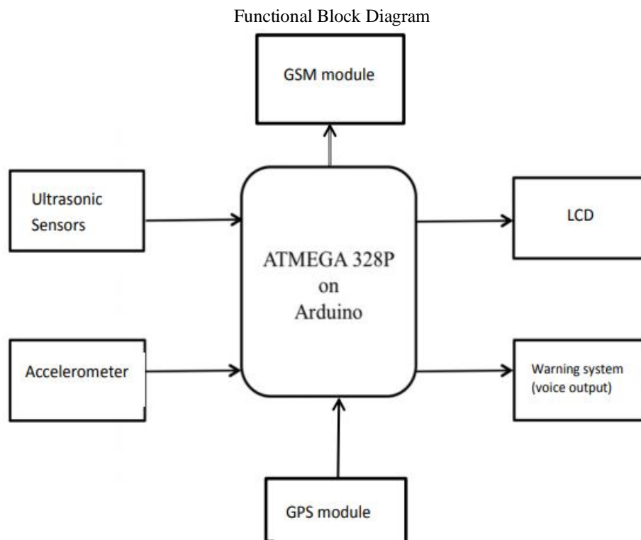
Figure 2: Block Diagram of Proposed System
