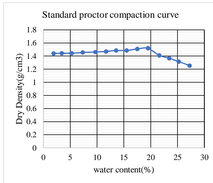
Fig 2: Variation of OMC and MDD for marine soil
