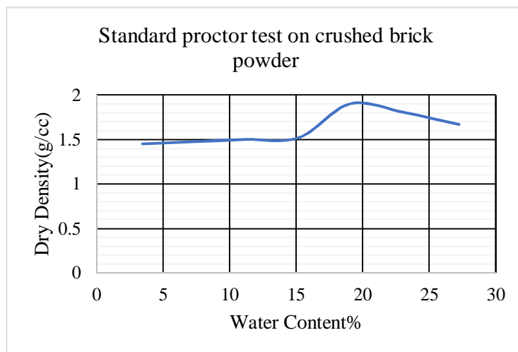
Fig 4: Compaction curve for brick powder
