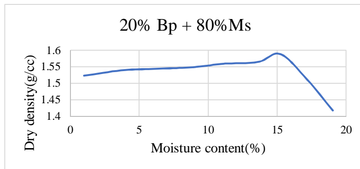
Fig 5: Graph of DD and MC for 20% Bp and 80% Ms
