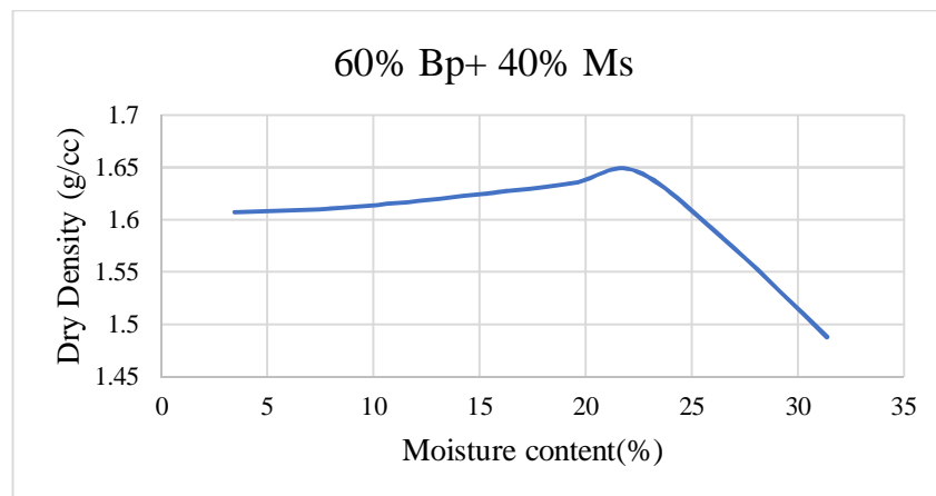
Fig 7: Graph of MD and MC for 60% Bp and 40% Ms
