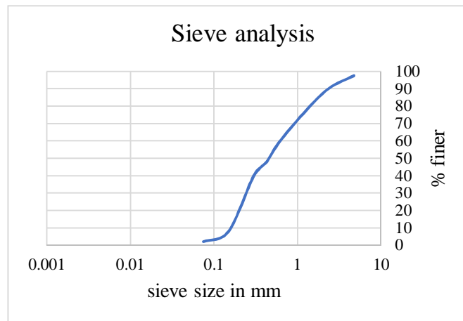
Fig 3: Particle size distribution curve for brick powder
