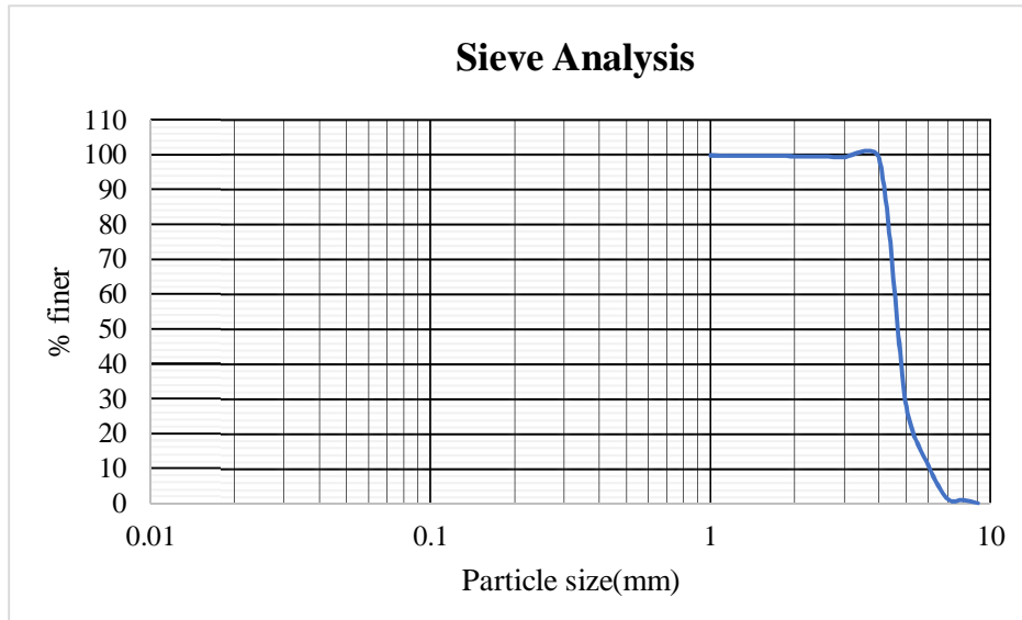
Figure 1 Grain size distribution curve for marine soil
