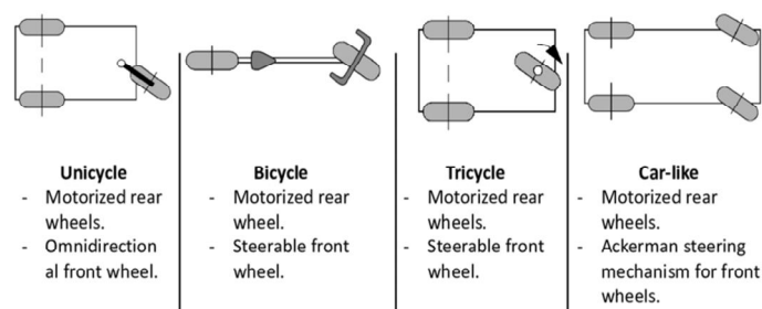
Fig. 1 Types of steering mechanisms
