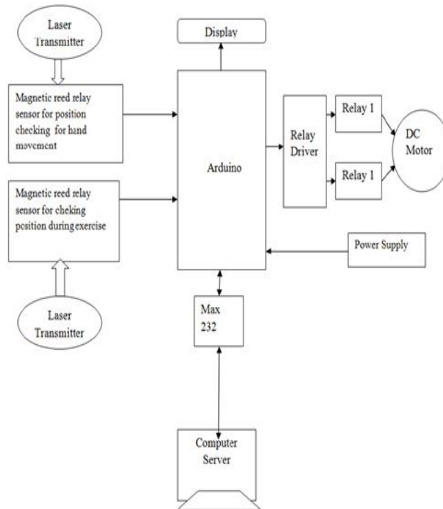
Figure. Arm exerciser model
