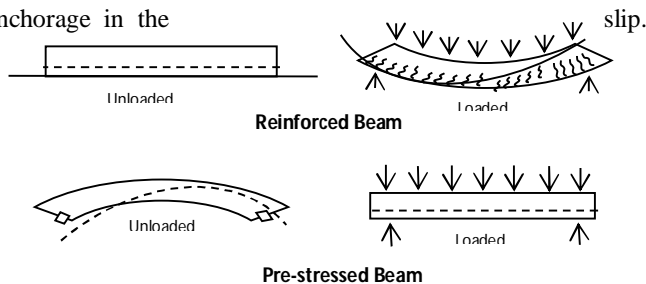
Fig. 2 PSC and RC behaviour after loading
