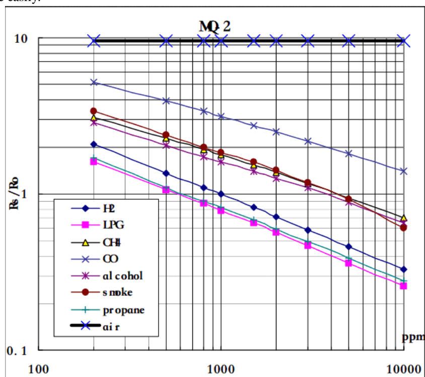
Fig.5 : Graph showing sensitivity curve of MQ2 Gas Sensor
