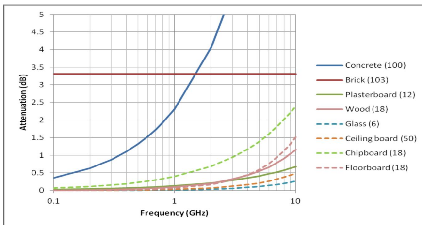
Fig 2: Attenuation of building material MMW (thickness in mm shown in legend) [7]
