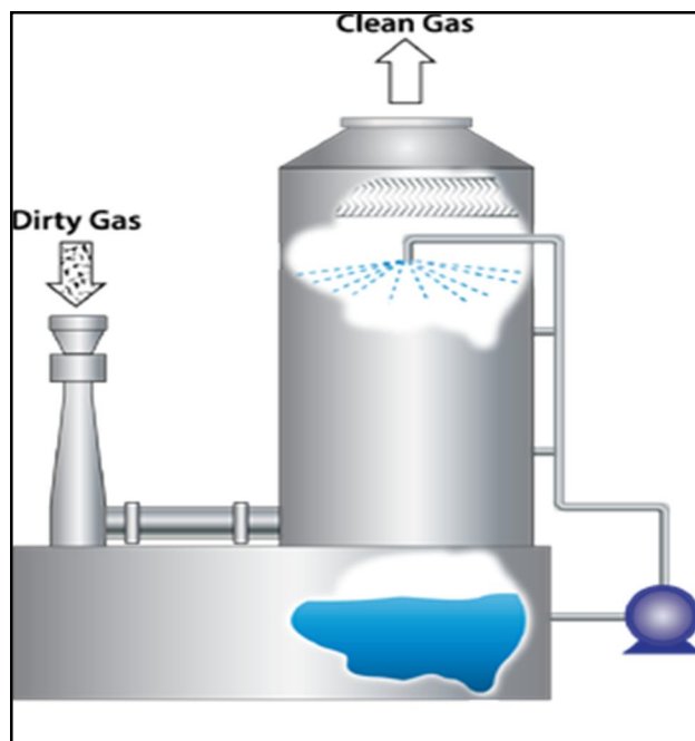
Fig: Wet Scrubber System
