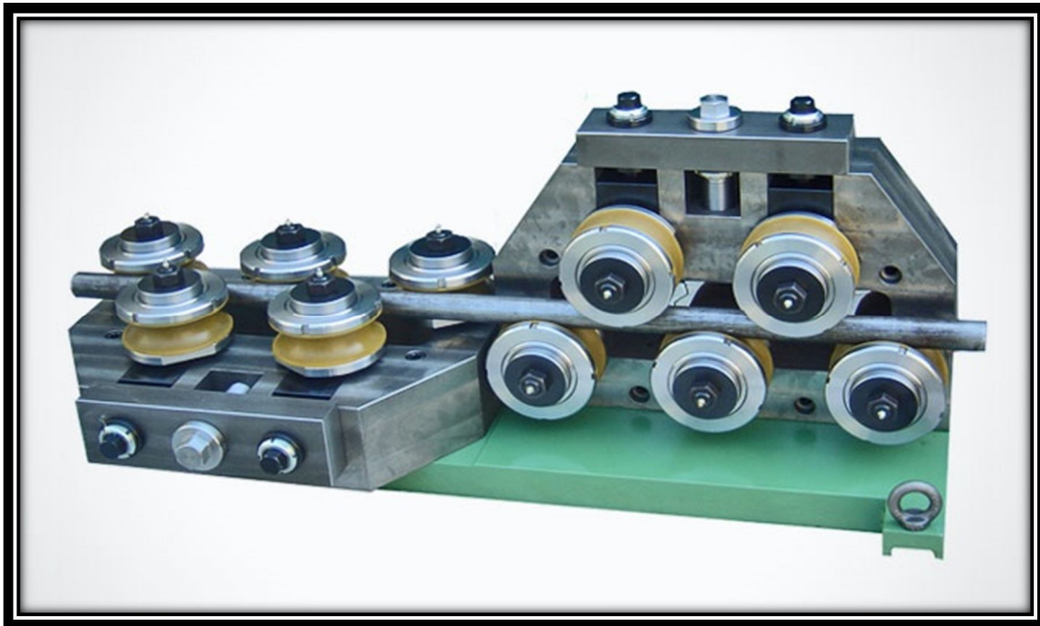
Fig 2: Mechanical Straightening
