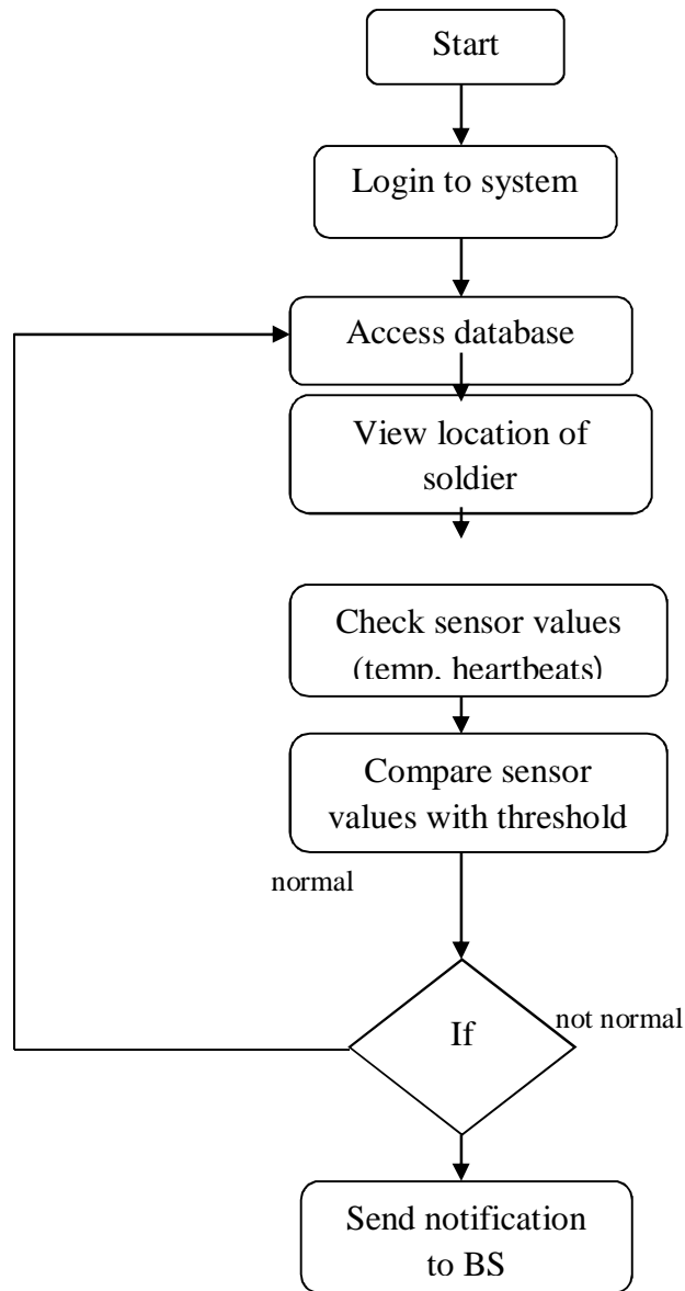
Fig (5.2) : Flow chart
