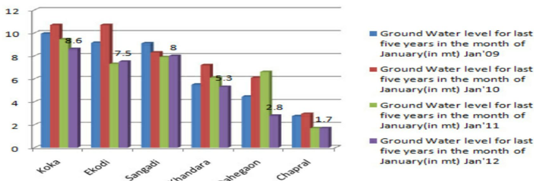
Figure 2 Ground Water Level in Various District of Maharashtra.
