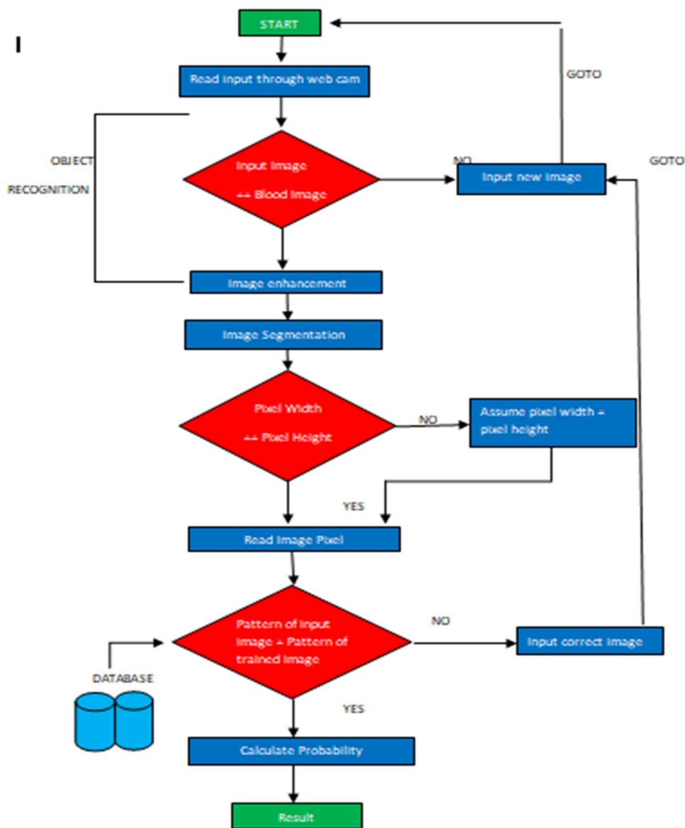
Figure 1. Flow chart of the Mechanism
