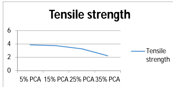
Chart3:- Tensile strength
