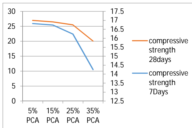
Chart2:- Compressive strength
