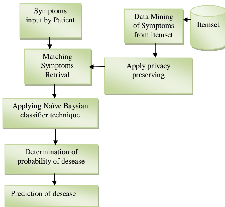
Fig. 1: Flow diagram of working System
