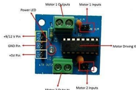
Fig.5 motor driver
