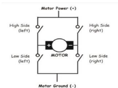
Fig.6 H-Bridge
