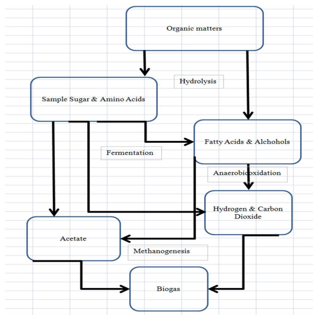
Fig-2 Process flow diagram for Anaerobic Digestion
