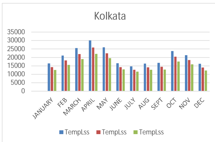
Figure 7. Loss diagram for Kolkata
