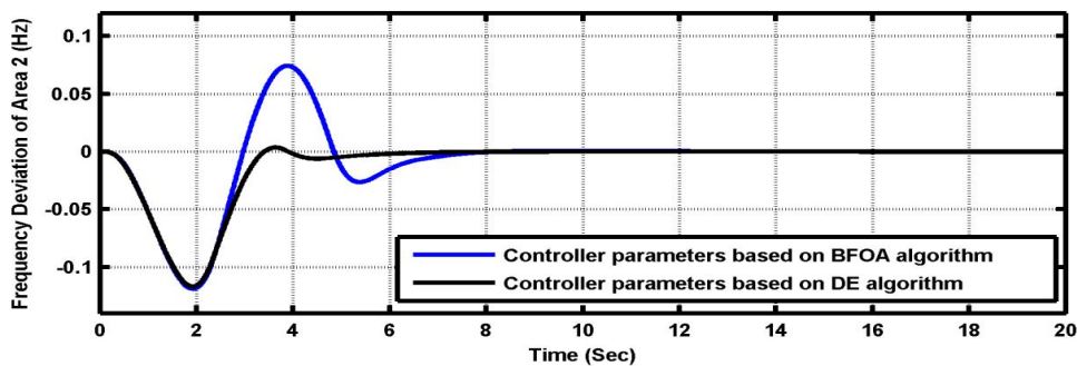
Fig. 14: Frequency Deviation of Area-2 for 5% step change in area-1 with 50% Decrease in T_{12} at \alpha=\pm 0.025
