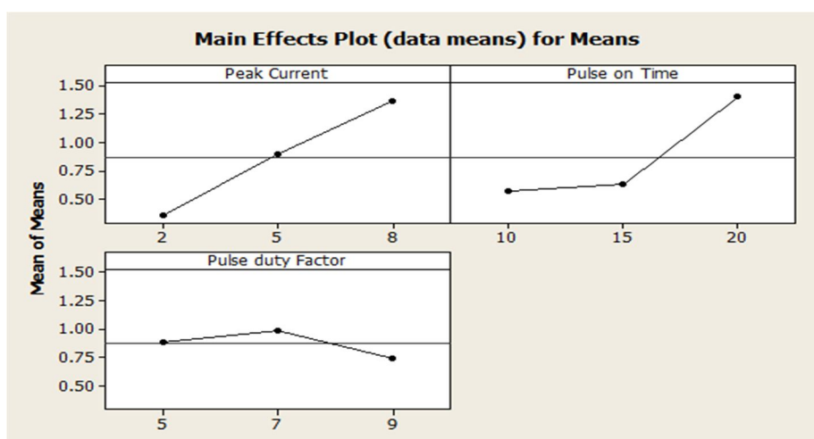
Fig. 2 Main effect plot for MRR
