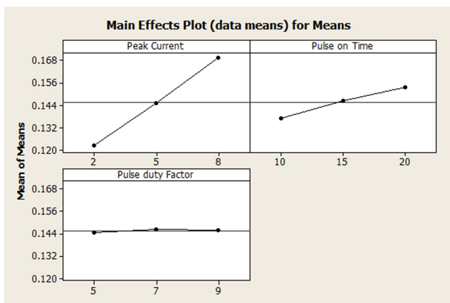
Fig. 5 Main effect plot for Radial Overcut
