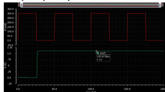
Figure 1.13 Transient response of wilson current mirror based level shifter
