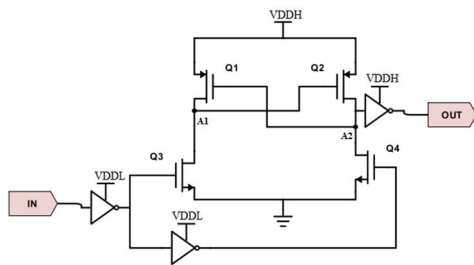
Figure 1.6 Circuit diagram of 10T DCVS based level shifter
