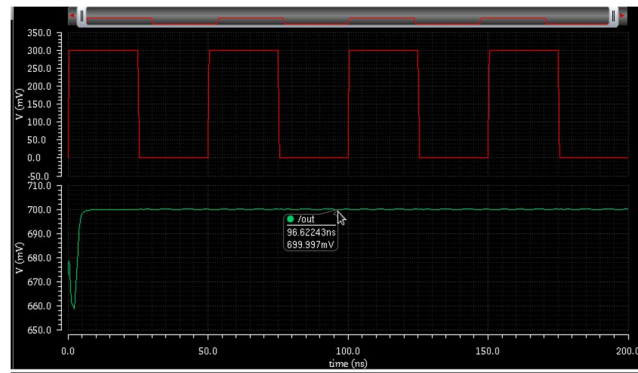
Figure 1.3 Transient response of 6T DCVS based level shifter
