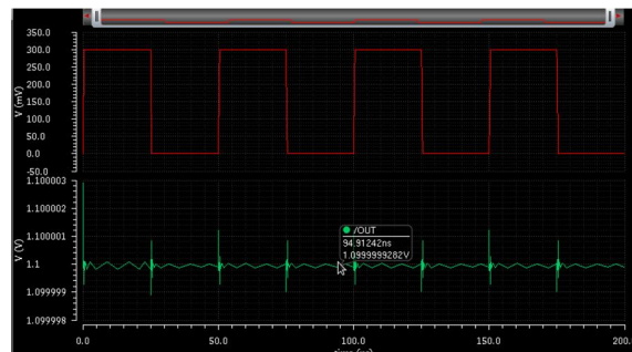
Figure 1.11 Transient response of current mirror based level shifter
