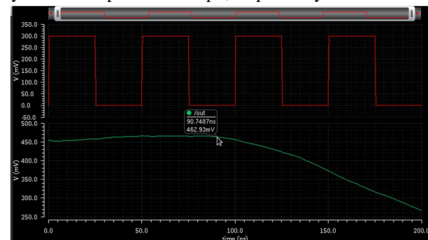
Figure 1.5 Transient response of 8T DCVS based level shifter
