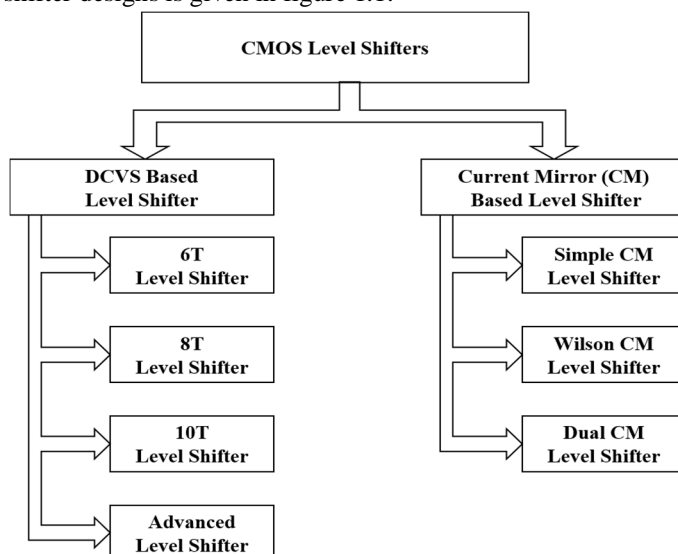
Figure 1.1 Classification of level shifter designs
