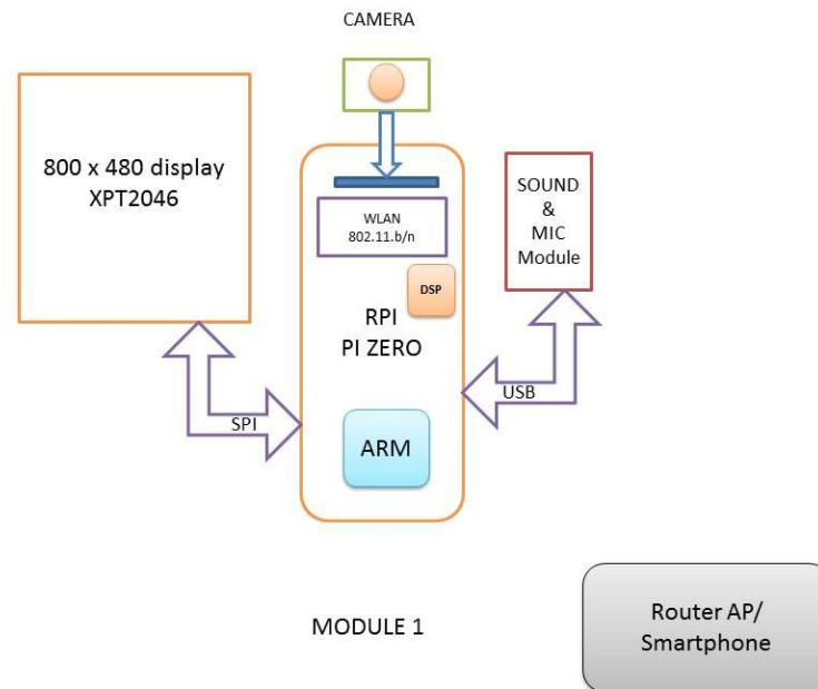
Fig. 1 Block Diagram of Digital Walkie-Talkie
