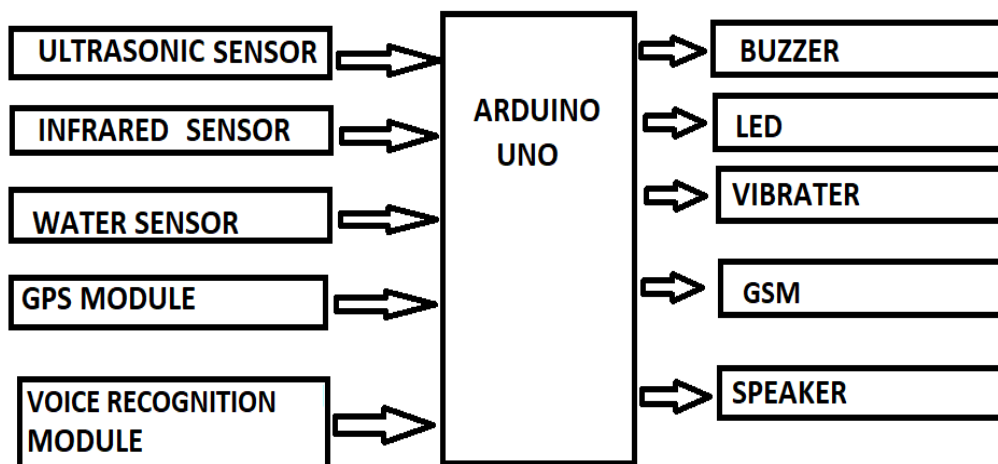
Fig. I: Block Diagram of Smart Blind Stick
