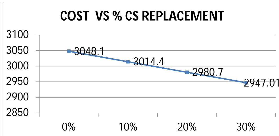
Graph 4.3 Cost (Rs.) per cubic m of concrete v/s % CS replacement
