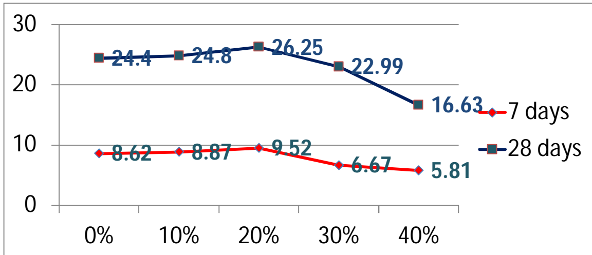
Graph 4.1 Compression Strength (MPa) v/s % CS replacements
