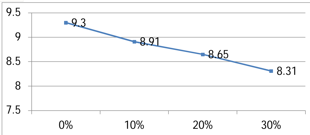
Graph 4.2 Weight of cube (Kg) v/s % CS replacement
