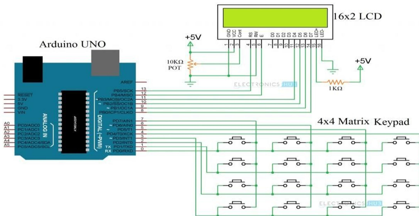
Interfacing of 4x4 Matrix keypad,16x2 LCD display and Audrino microcontroller ATMEL 2560
