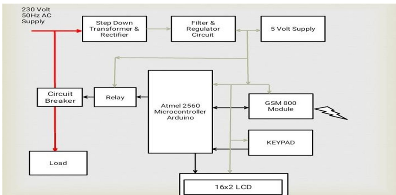
Block Diagram of password based circuit breaker using GSM MODULE
