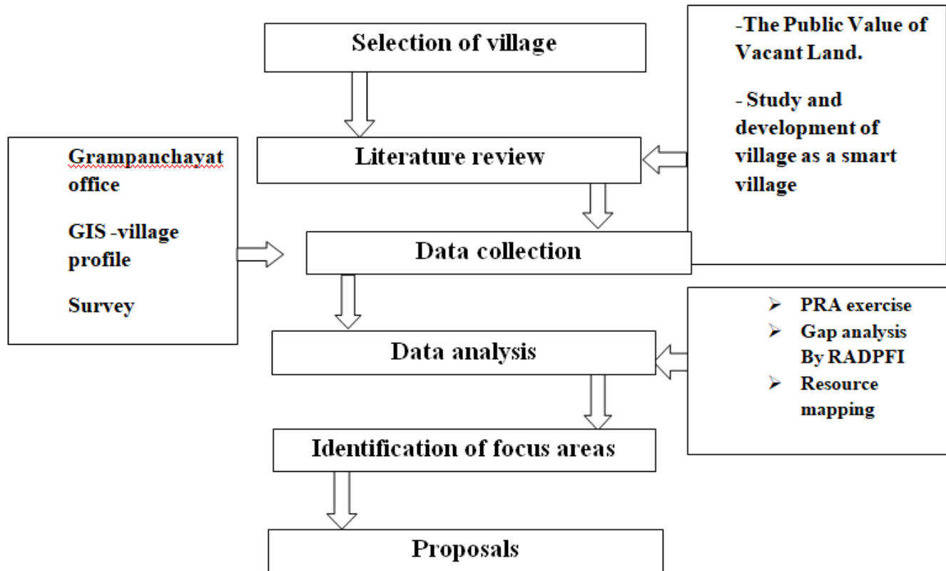
Figure 2 methodology chart.
