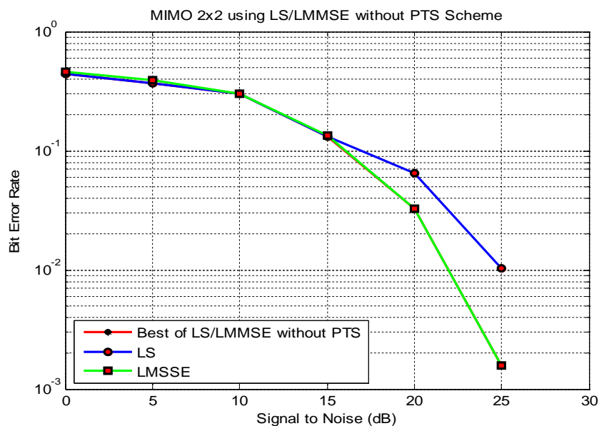
Figure 4 -Performance of 2x2 MIMO-OFDM system using LS/LMMSE with PTS scheme
