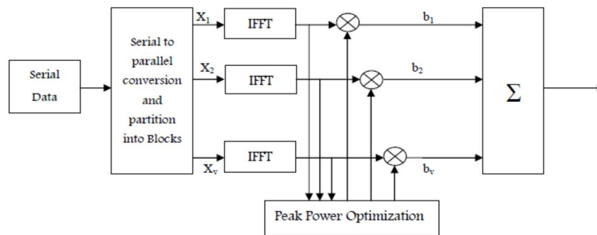
Figure 2- Block Diagram of PTS scheme
