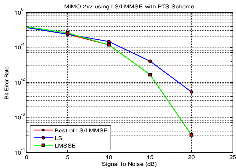
Figure 3-Performance of 2x2 MIMO-OFDM system using LS/LMMSE without PTS scheme
