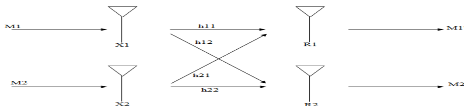
Figure 1- Transmit and Receive (2x2) MIMO System with channel coefficients
