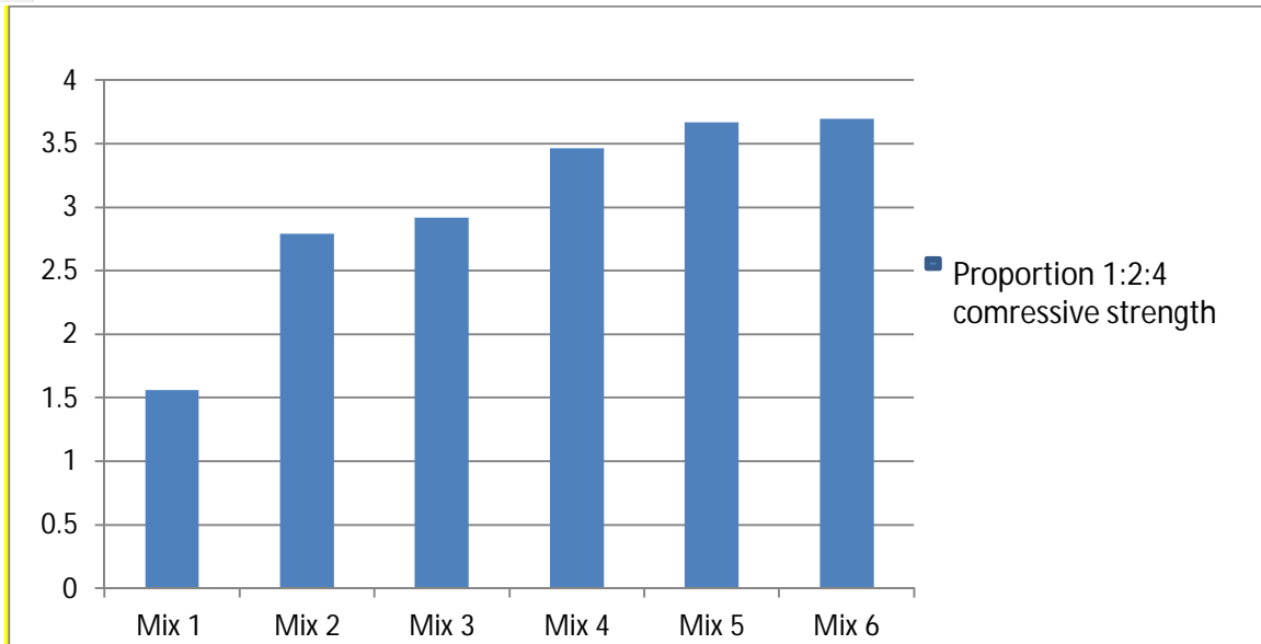
Fig.1 compression test result for 14 days
