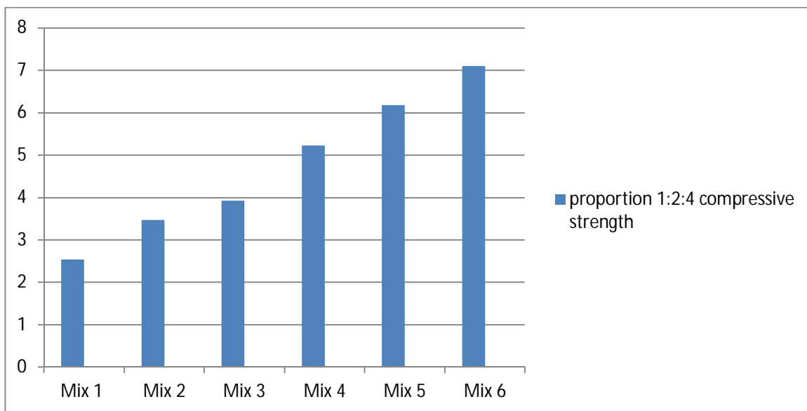
Fig.2 compression test result for 28 days
