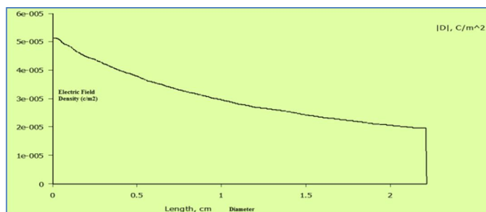
Fig.8. Electric field Density of EPR based 33kV cable using FEM in radial direction
