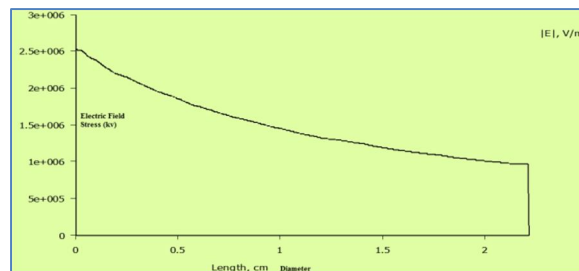
Fig.7. Electric field stress of EPR based 33kV cable using FEM in radial direction.
