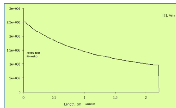
Fig.4. Electric field stress of XLPE based 33kV cable using FEM in radial direction
