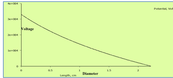
Fig.3. Voltage Distribution of XLPE based 33kV cable Using FEM in radial direction
