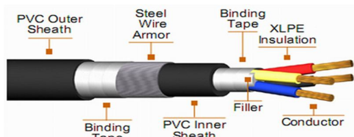
Fig.1. Detail View of High Voltage (HV) underground cable
