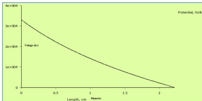
Fig.6. Voltage Distribution of EPR based 33kV cable using FEM in radial direction
