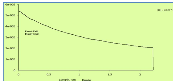
Fig.5. Electric field Density of XLPE based 33kV cable using FEM in radial direction
