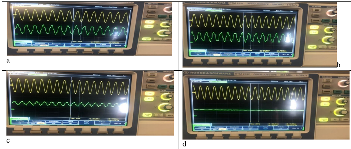
Fig. 7. lowpass filter prototype of (a) Input at 70Hz (b) Input Signal at 75Hz (c) Input Signal at 80Hz (d) Input Signal at 80Hz
