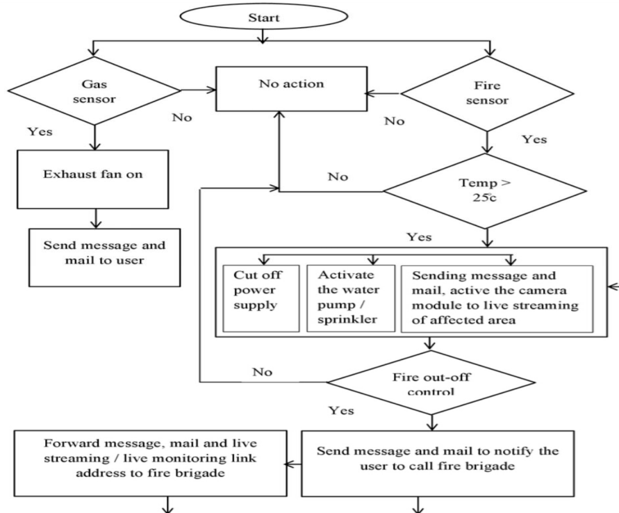
Fig 3: proposed system flowchart
