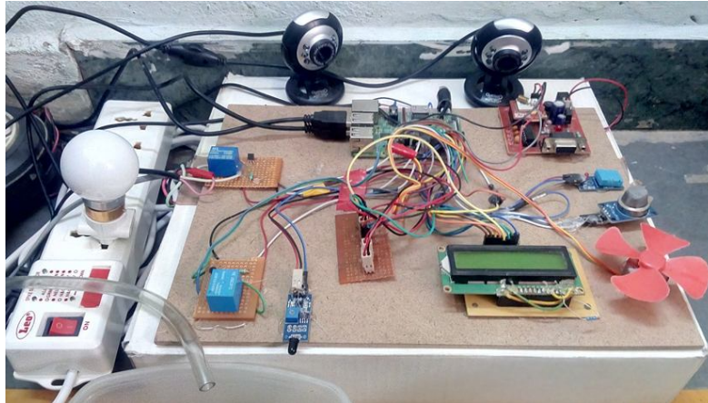
Fig 2: Picture of Implemented proposed system
