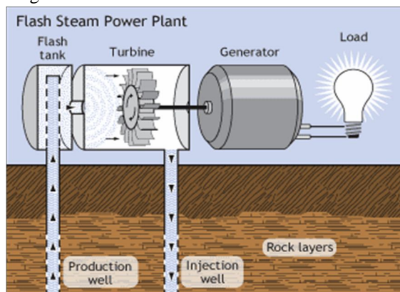
Fig. 3. Flash cycle
