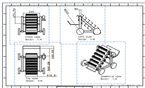
Fig.2. Drafted view of beach cleaning machine
