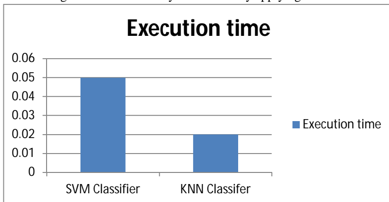
Fig 3: Execution Time
