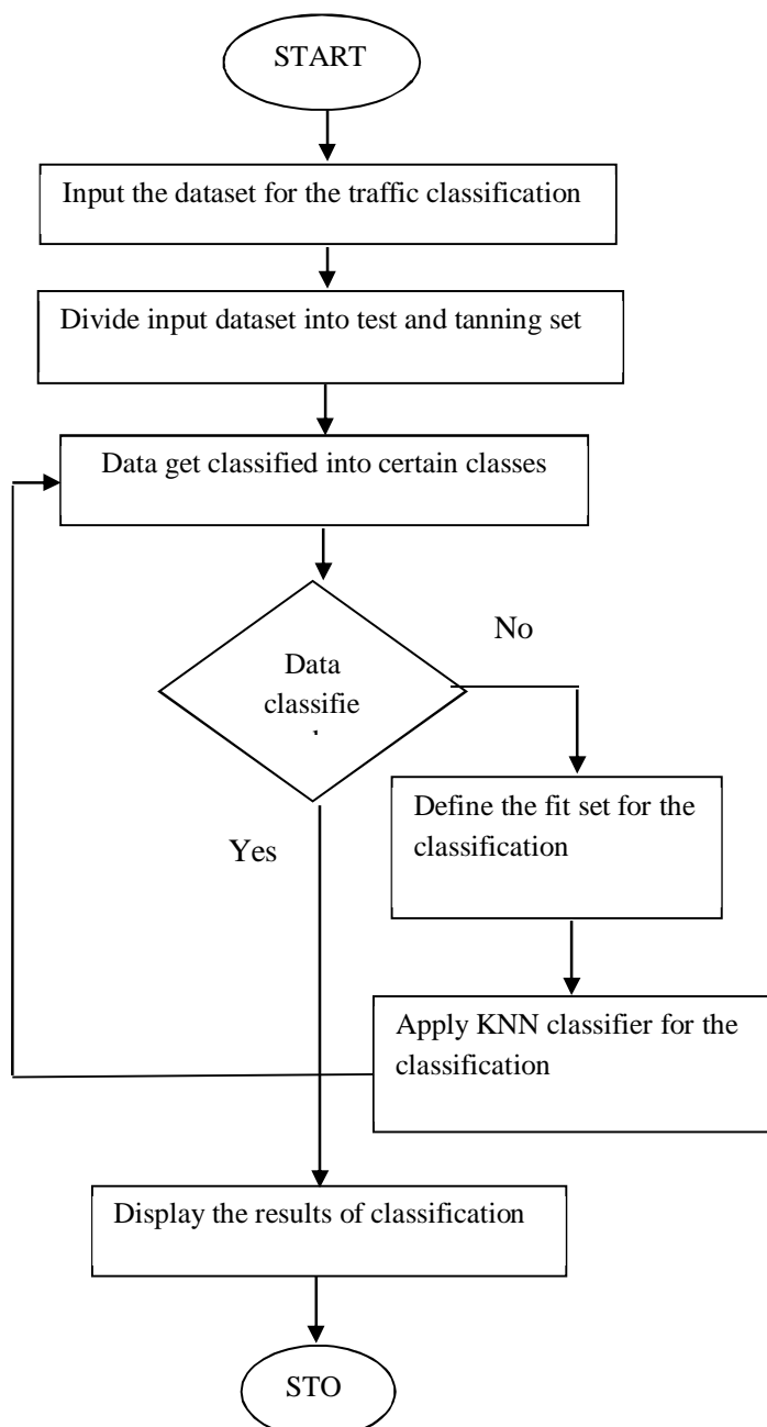
Figure 1: Proposed Flowchart
