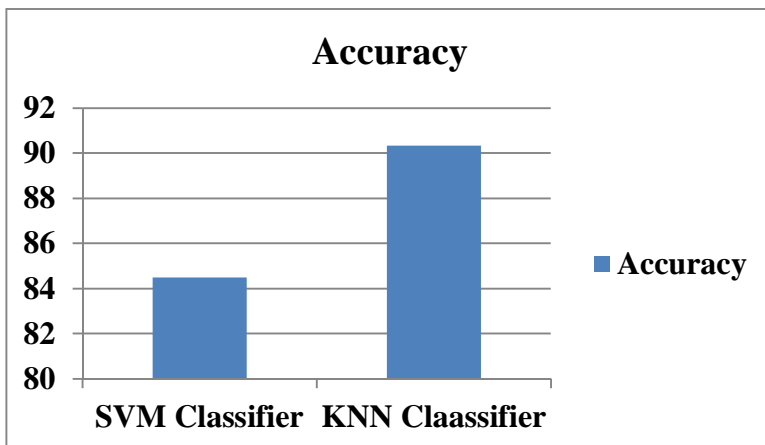
Fig 2: Accuracy Comparison
