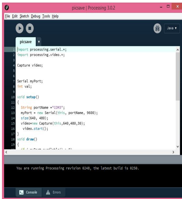
Fig. 4.Processing IDE window
