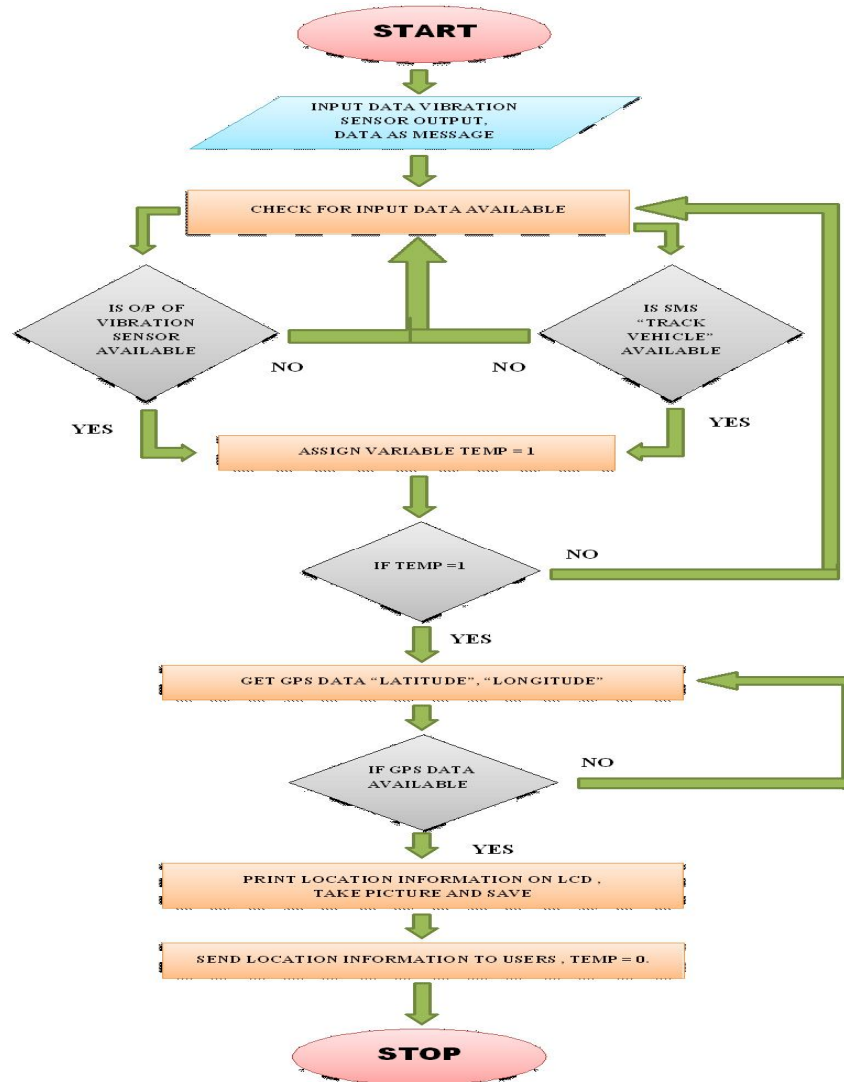
Fig. 5. Flow chart of device working
