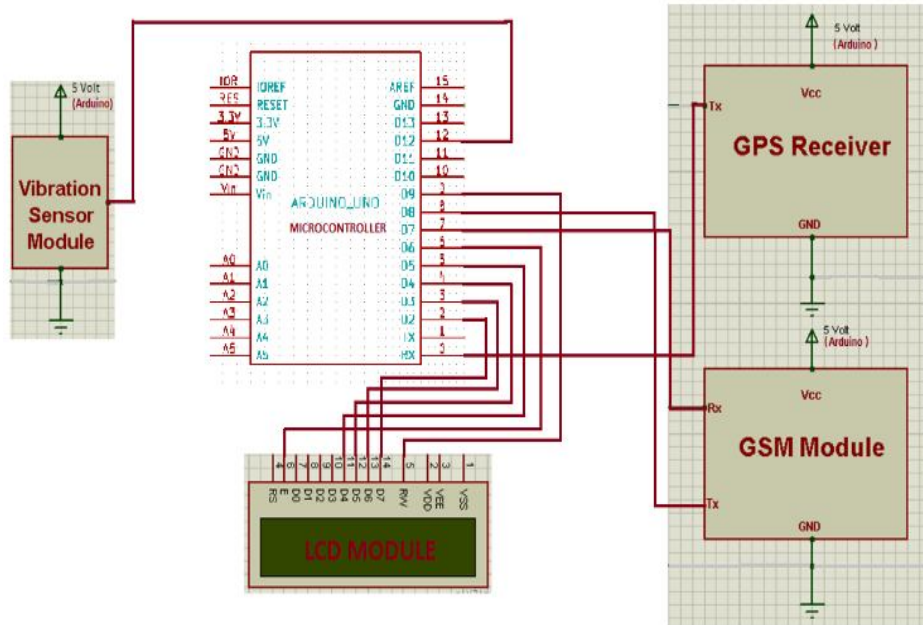
Fig. 1. Circuit diagram
