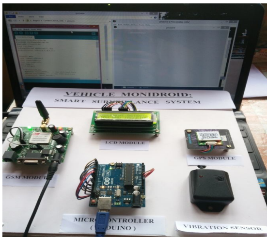
Fig. 6. Working pictures of module
