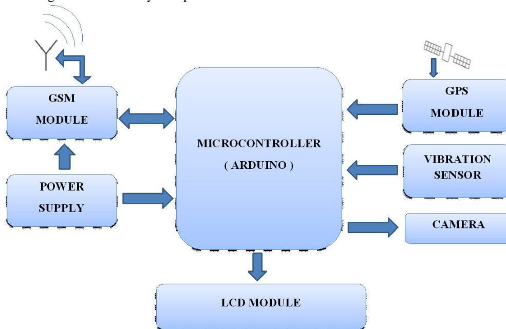
Fig. 2. Block diagram
